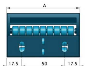
T-770SS
