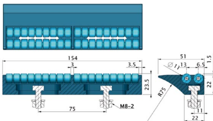
T-310SS
